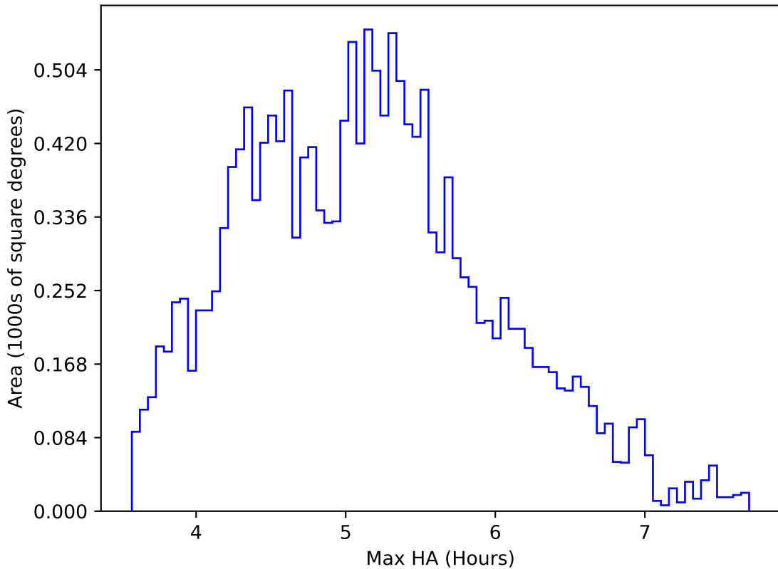
ddf_loaded_fl8_v3.4_10yrs WFD all bands: Max HA
