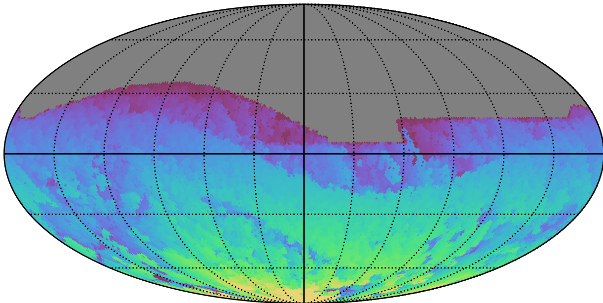
ddf_loaded_fl8_v3.4_10yrs All sky z band: Max HA
