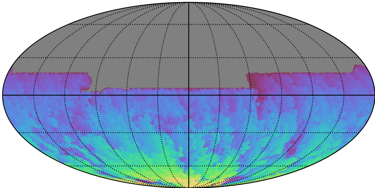
ddf_loaded_fl8_v3.4_10yrs All sky y band: Max HA
