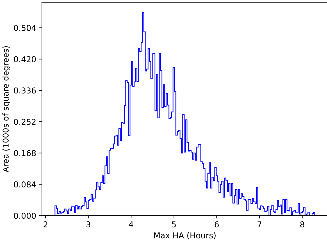
ddf_loaded_fl8_v3.4_10yrs All sky y band: Max HA
