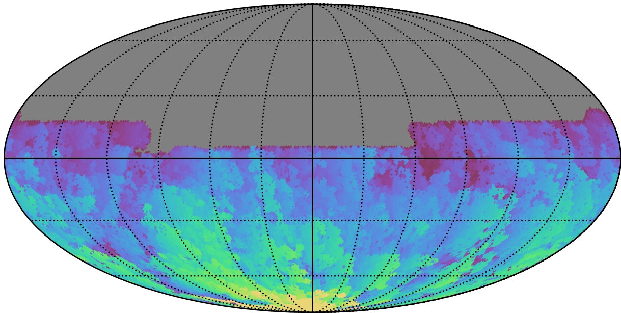
ddf_loaded_fl8_v3.4_10yrs All sky u band: Max HA
