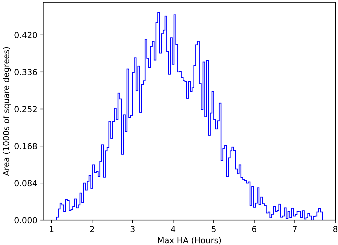
ddf_loaded_fl8_v3.4_10yrs All sky u band: Max HA
