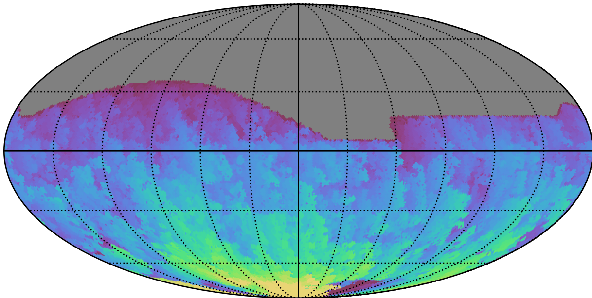
ddf_loaded_fl8_v3.4_10yrs All sky r band: Max HA
