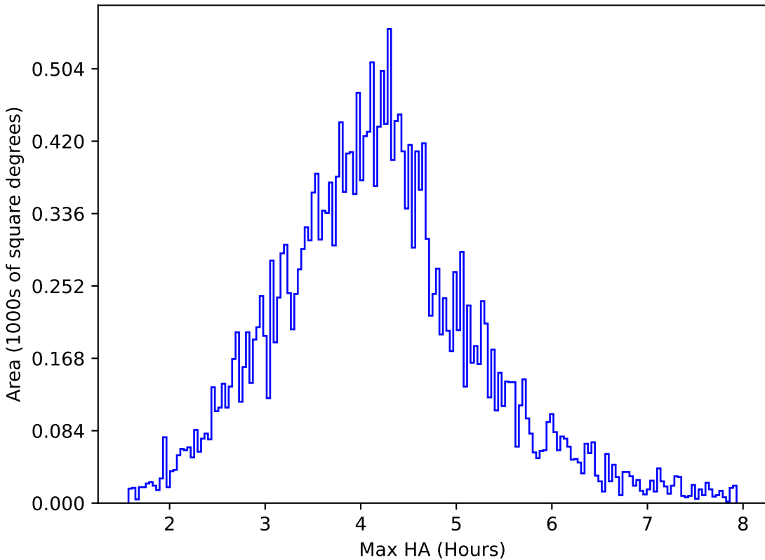
ddf_loaded_fl8_v3.4_10yrs All sky r band: Max HA
