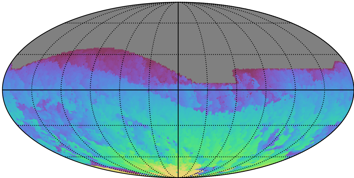
ddf_loaded_fl8_v3.4_10yrs All sky i band: Max HA
