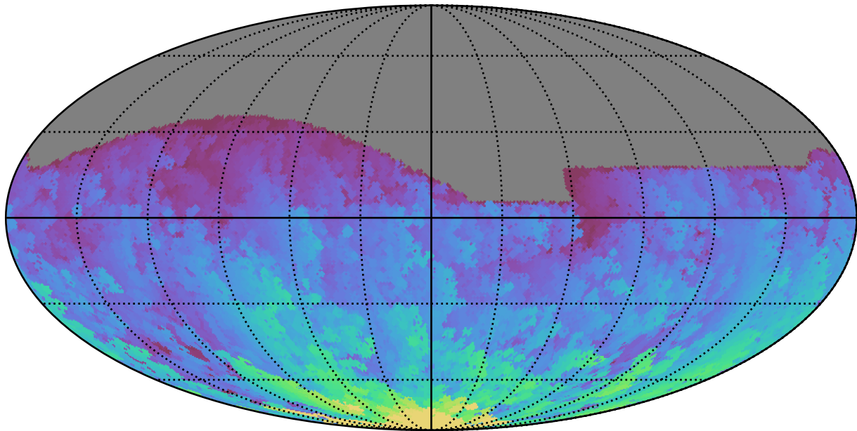
ddf_loaded_fl8_v3.4_10yrs All sky g band: Max HA
