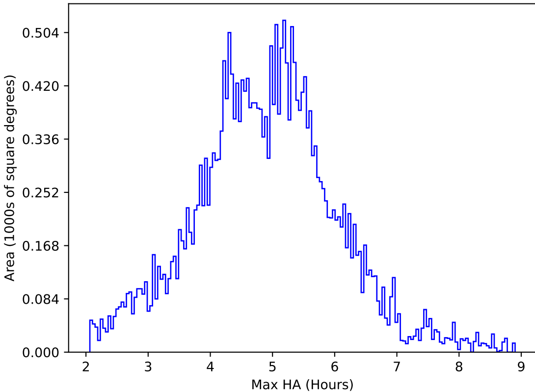
ddf_loaded_fl8_v3.4_10yrs All sky all bands: Max HA
