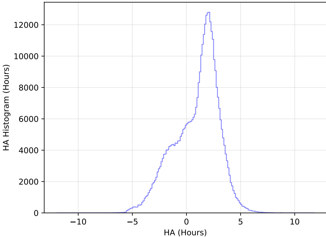
ddf_loaded_fl8_v3.4_10yrs WFD y band: HA Histogram
