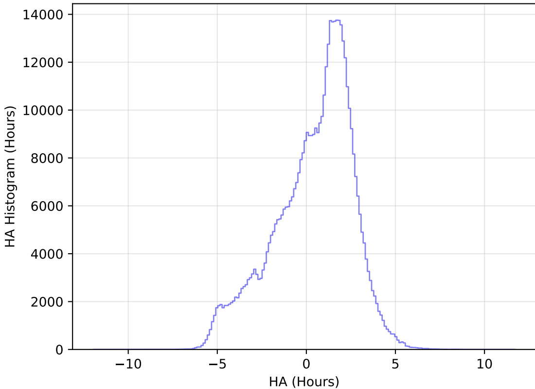
ddf_loaded_fl8_v3.4_10yrs WFD r band: HA Histogram
