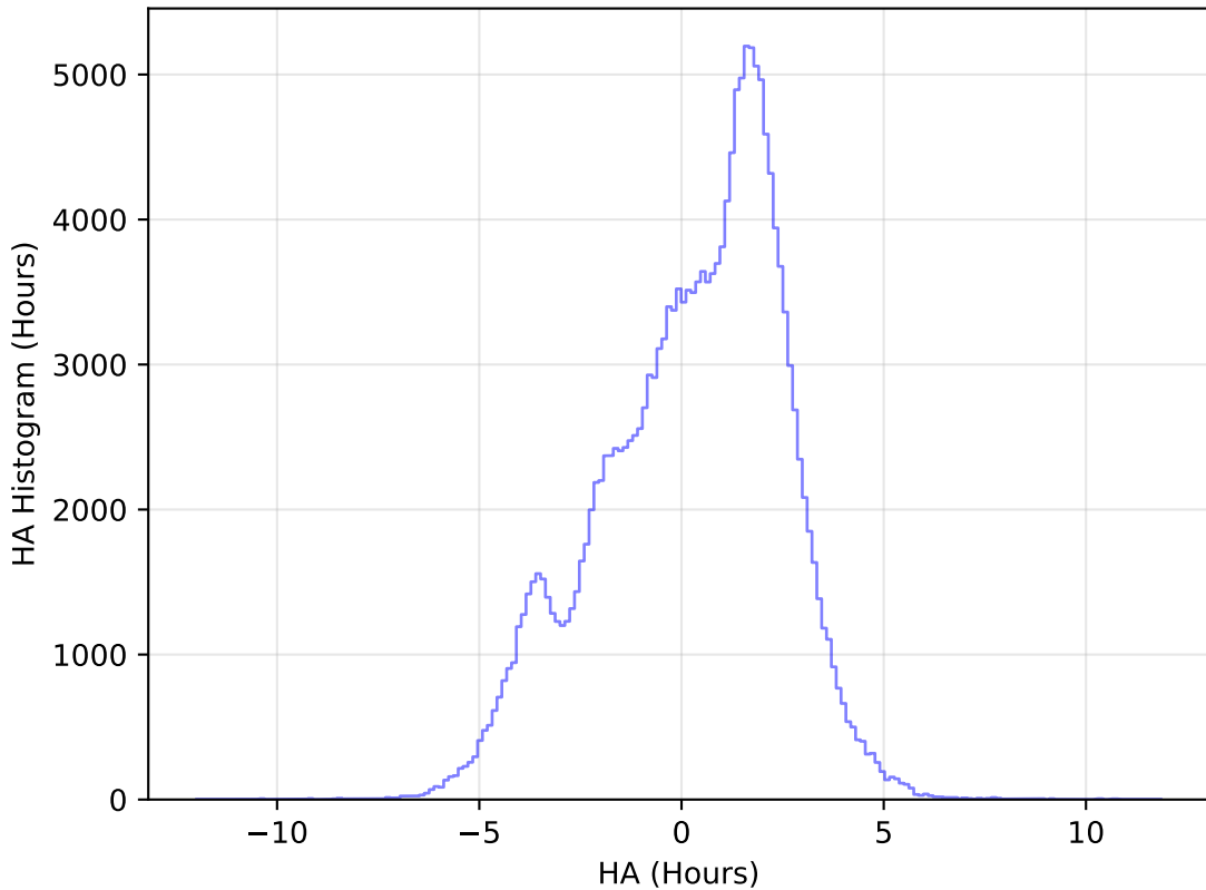
ddf_loaded_fl8_v3.4_10yrs WFD g band: HA Histogram
