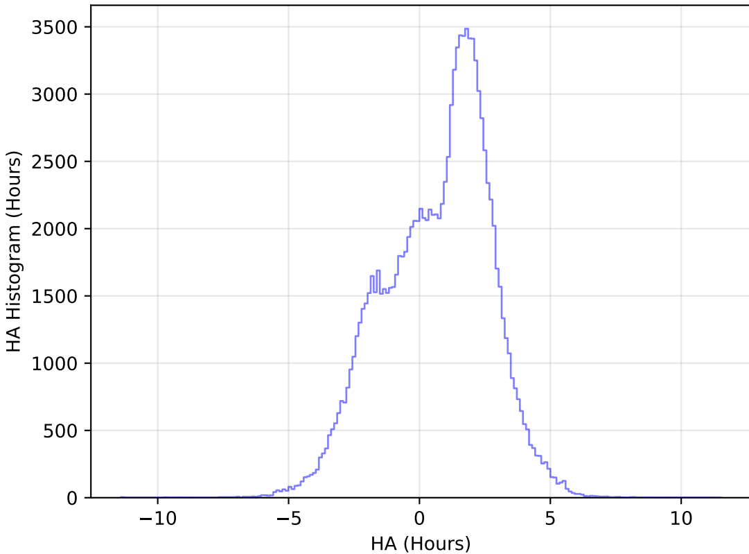
ddf_loaded_fl8_v3.4_10yrs All sky u band: HA Histogram
