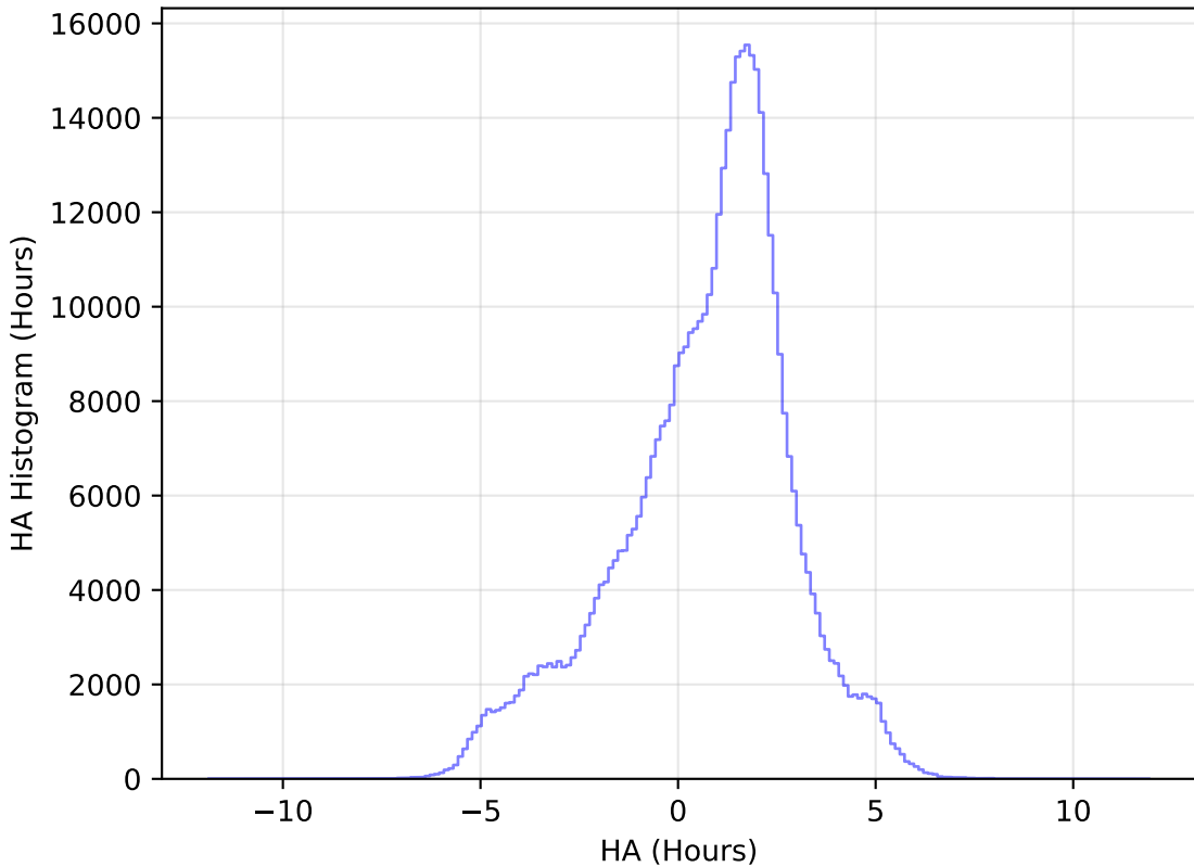
ddf_loaded_fl8_v3.4_10yrs All sky i band: HA Histogram
