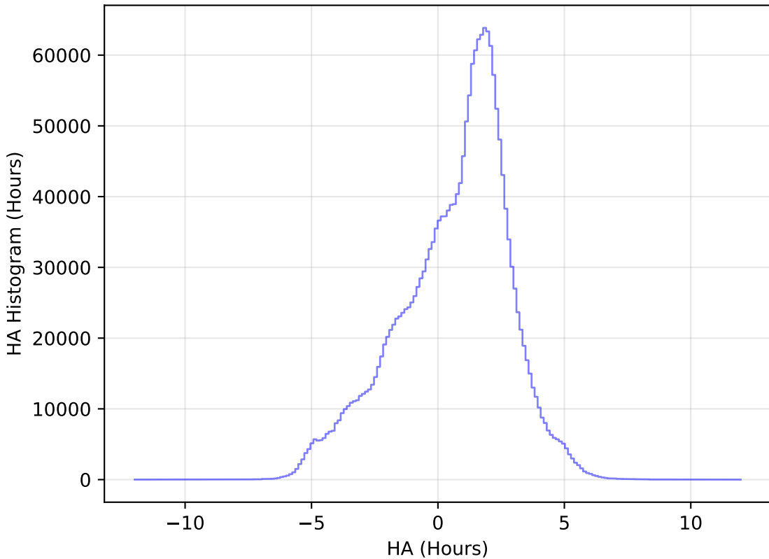
ddf_loaded_fl8_v3.4_10yrs All sky all bands: HA Histogram
