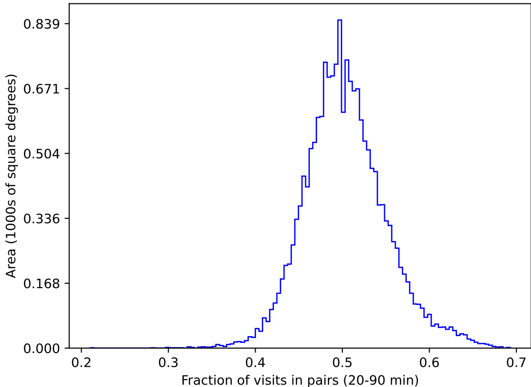
ddf_loaded_fl8_v3.4_10yrs gri WFD: Fraction of visits in pairs (20-90 min)
