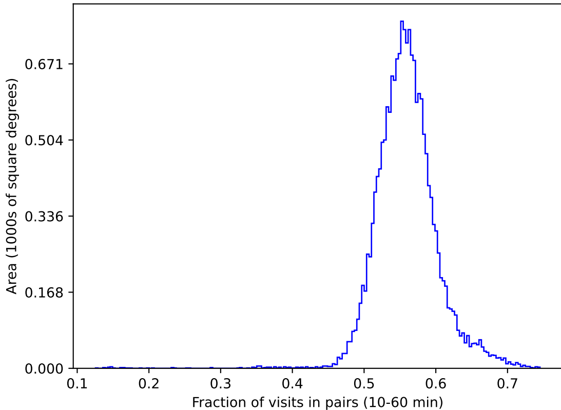
ddf_loaded_fl8_v3.4_10yrs gri WFD: Fraction of visits in pairs (10-60 min)
