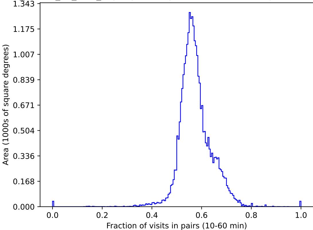
ddf_loaded_fl8_v3.4_10yrs gri All sky: Fraction of visits in pairs (10-60 min)
