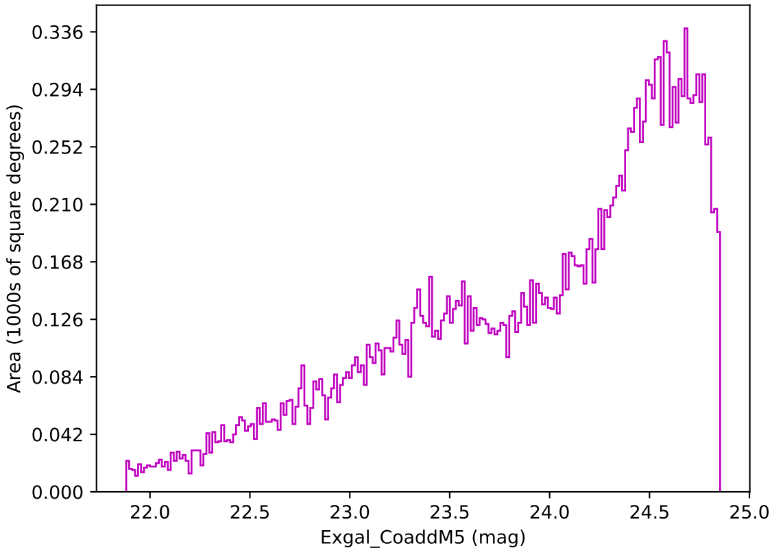
ddf_loaded_fl8_v3.4_10yrs Yr 3-4 z band: Exgal_CoaddM5
