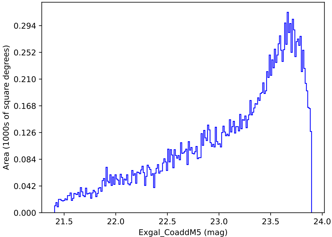
ddf_loaded_fl8_v3.4_10yrs Yr 3-4 y band: Exgal_CoaddM5
