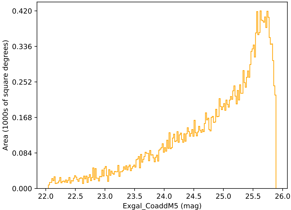
ddf_loaded_fl8_v3.4_10yrs Yr 3-4 r band: Exgal_CoaddM5
