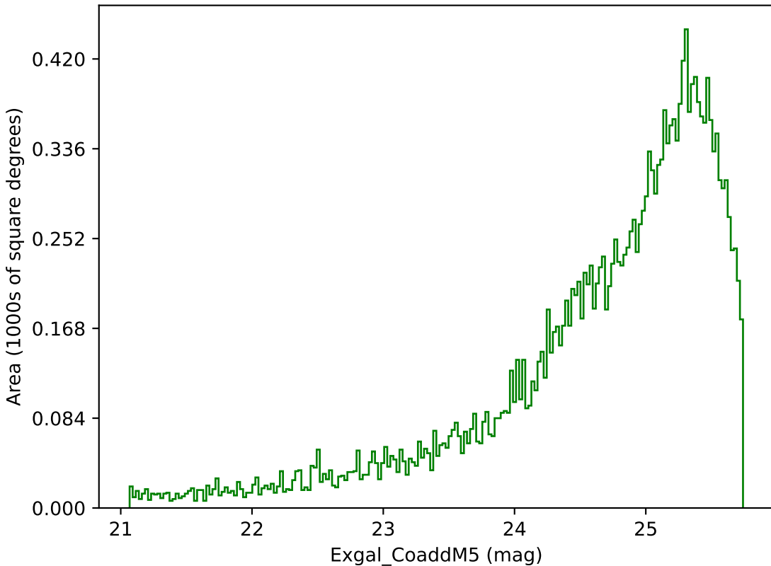
ddf_loaded_fl8_v3.4_10yrs Yr 3-4 g band: Exgal_CoaddM5
