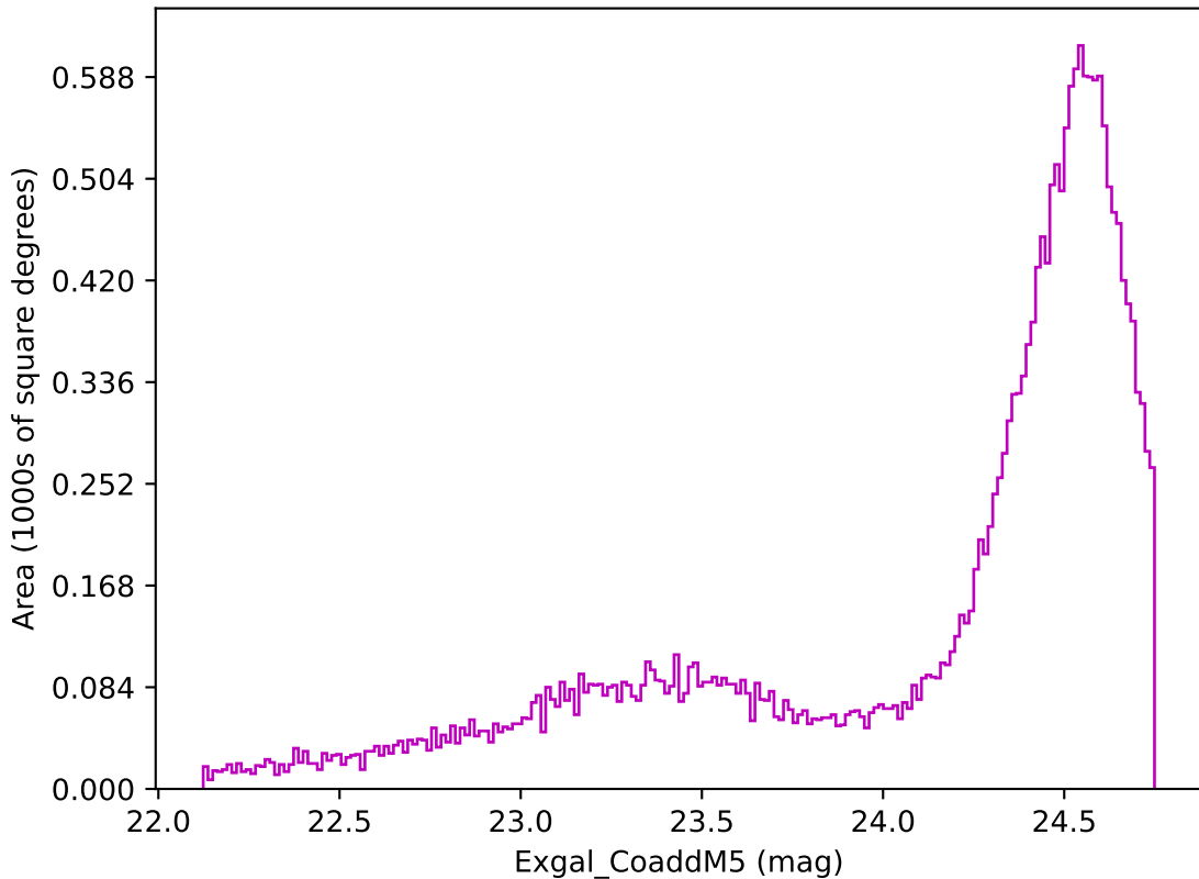
ddf_loaded_fl8_v3.4_10yrs Yr 1 z band: Exgal_CoaddM5
