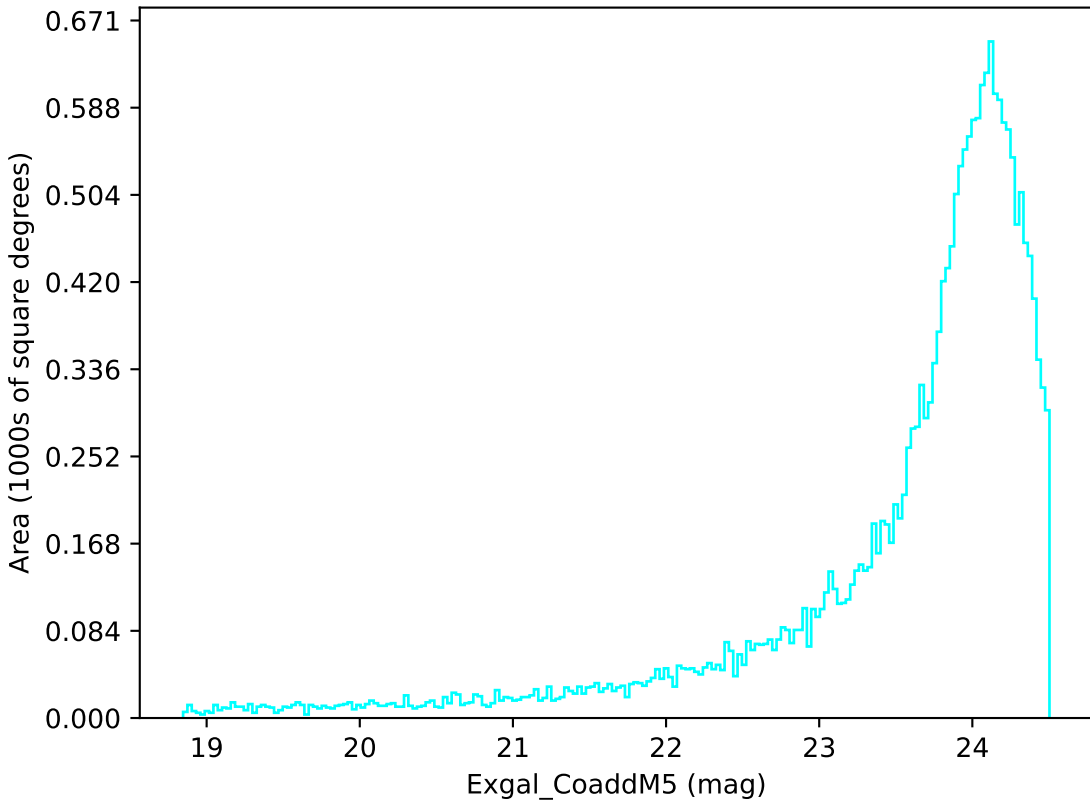
ddf_loaded_fl8_v3.4_10yrs Yr 1 u band: Exgal_CoaddM5
