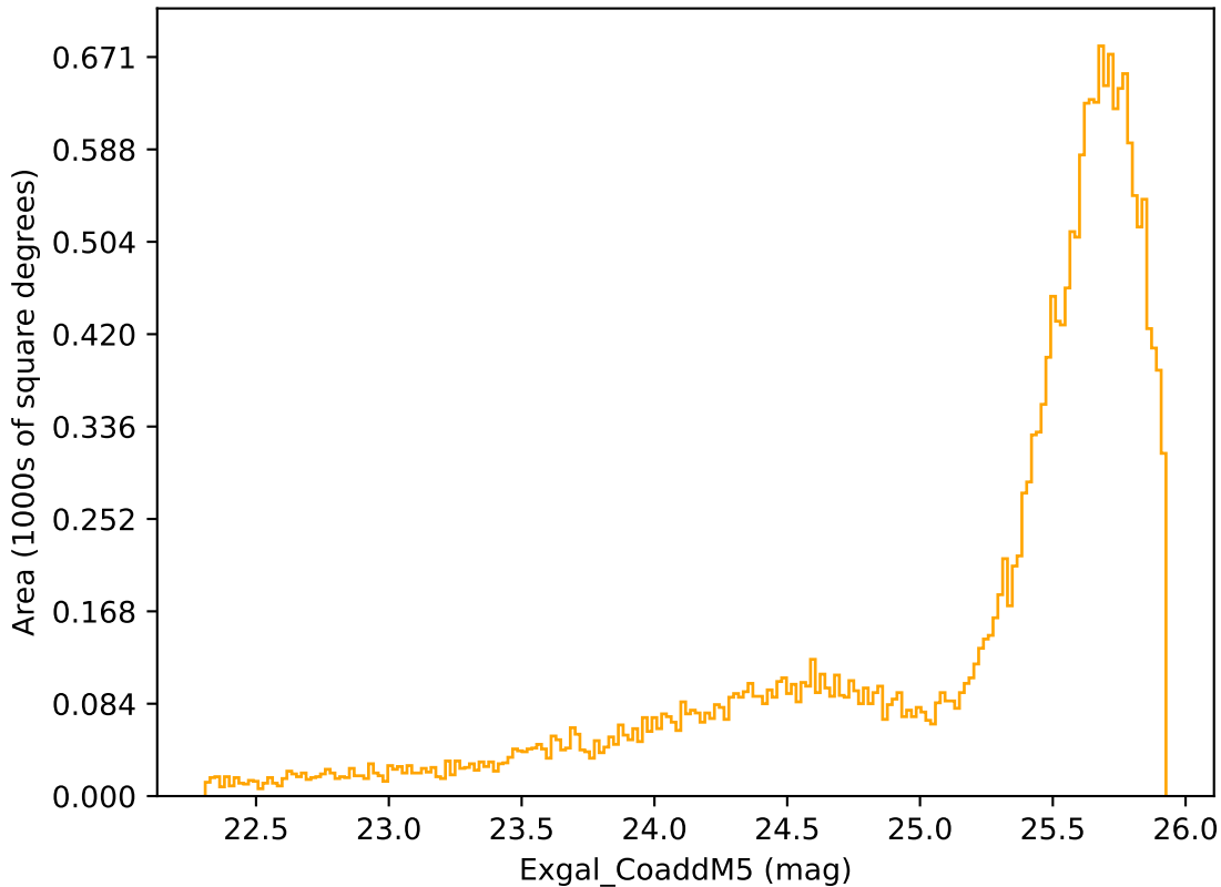
ddf_loaded_fl8_v3.4_10yrs Yr 1 r band: Exgal_CoaddM5
