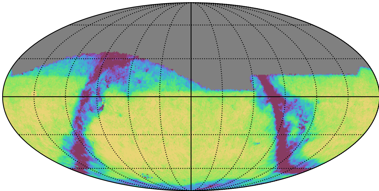
ddf_loaded_fl8_v3.4_10yrs Yr 1 i band: Exgal_CoaddM5
