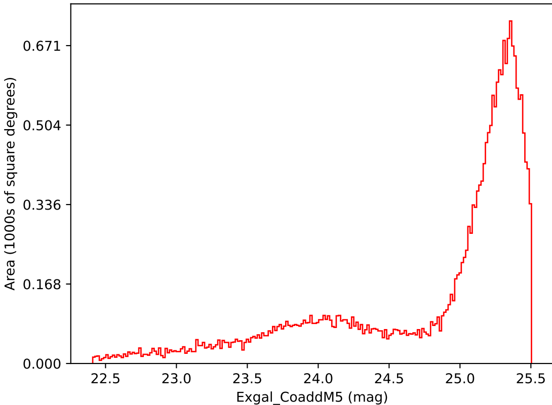
ddf_loaded_fl8_v3.4_10yrs Yr 1 i band: Exgal_CoaddM5
