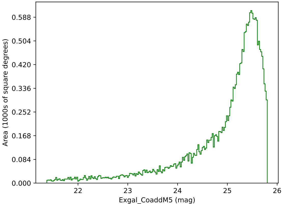
ddf_loaded_fl8_v3.4_10yrs Yr 1 g band: Exgal_CoaddM5
