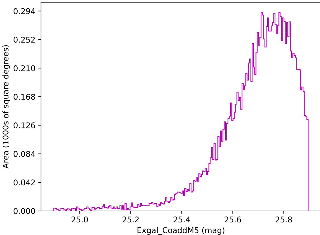
ddf_loaded_fl8_v3.4_10yrs WFD z band: Exgal_CoaddM5
