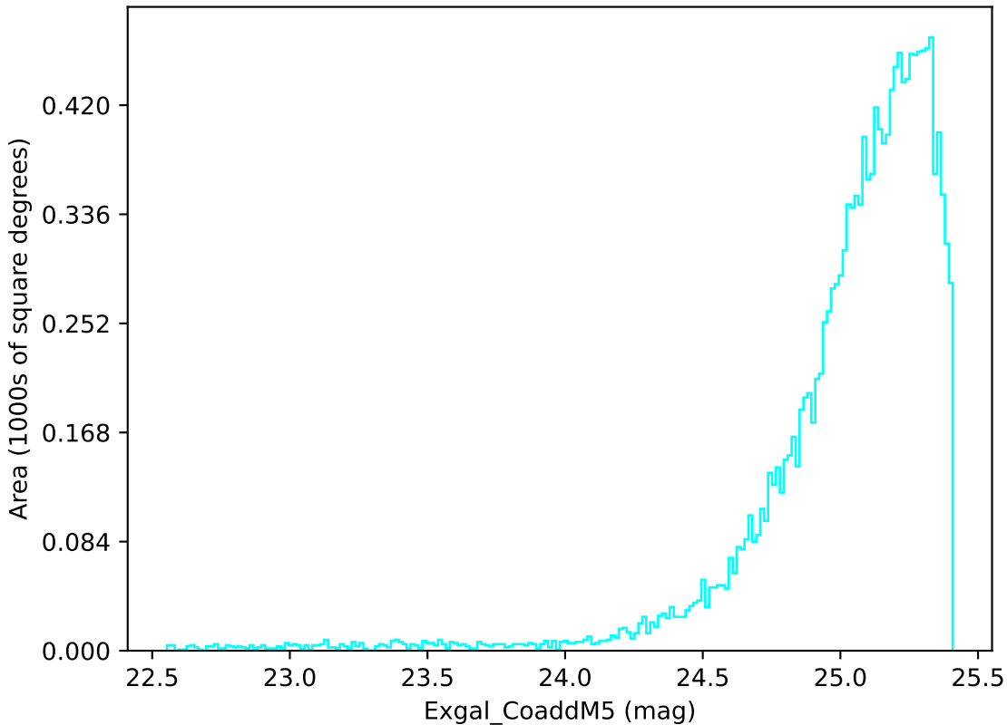
ddf_loaded_fl8_v3.4_10yrs WFD u band: Exgal_CoaddM5
