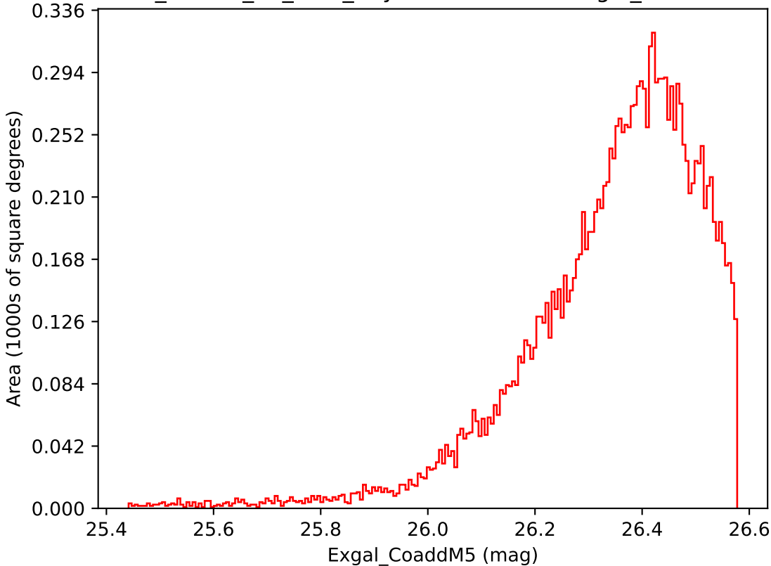
ddf_loaded_fl8_v3.4_10yrs WFD i band: Exgal_CoaddM5
