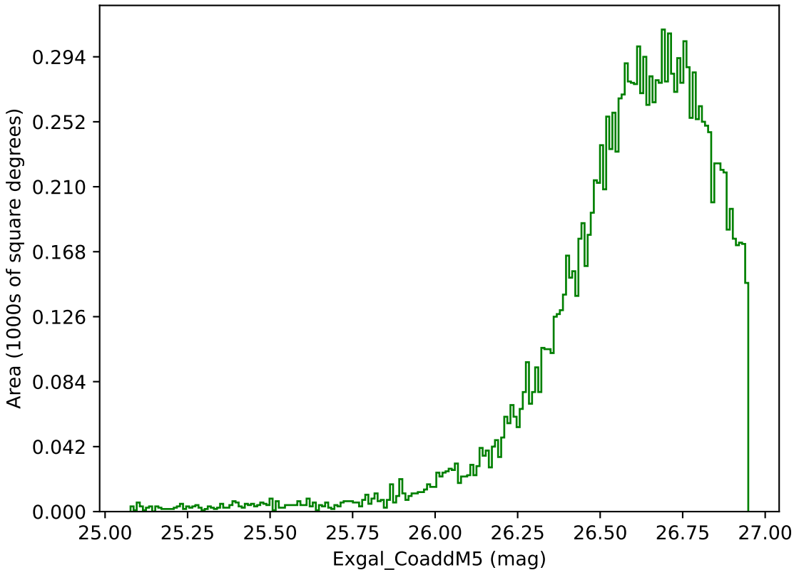
ddf_loaded_fl8_v3.4_10yrs WFD g band: Exgal_CoaddM5
