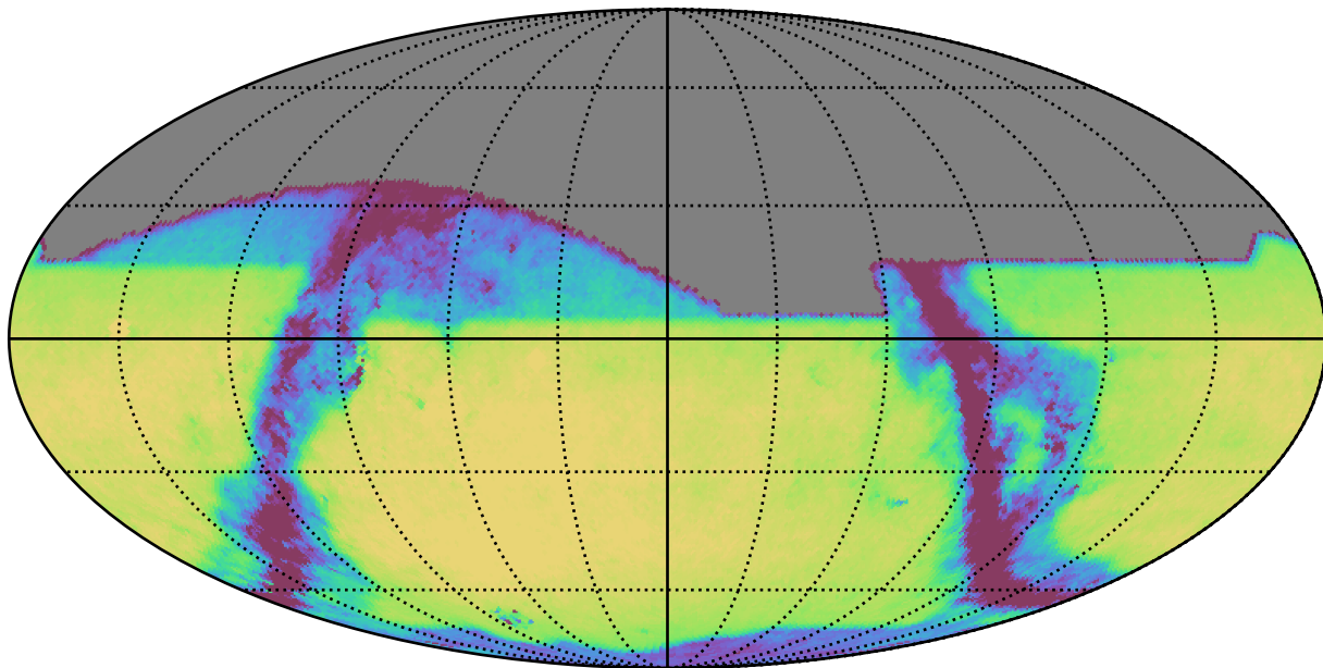
ddf_loaded_fl8_v3.4_10yrs All sky z band: Exgal_CoaddM5
