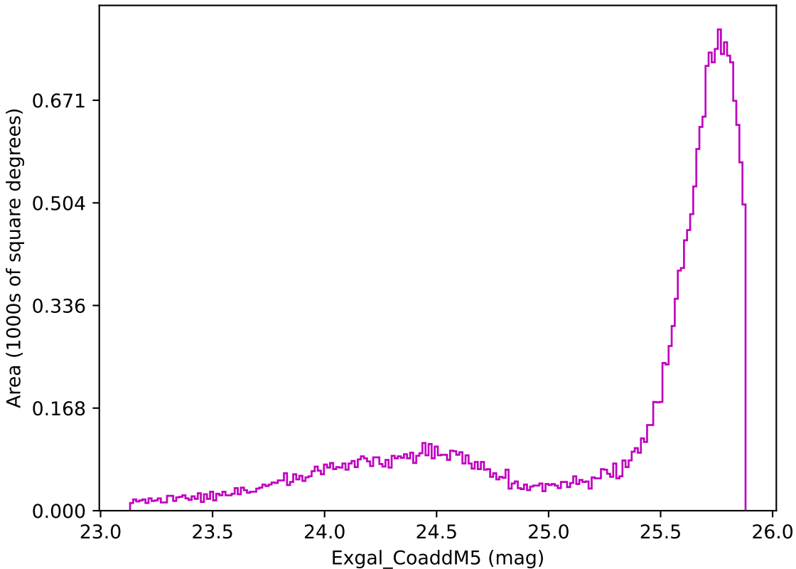
ddf_loaded_fl8_v3.4_10yrs All sky z band: Exgal_CoaddM5
