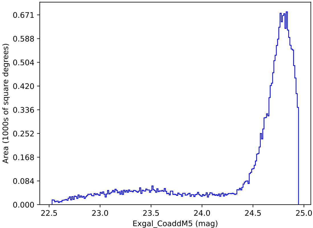
ddf_loaded_fl8_v3.4_10yrs All sky y band: Exgal_CoaddM5
