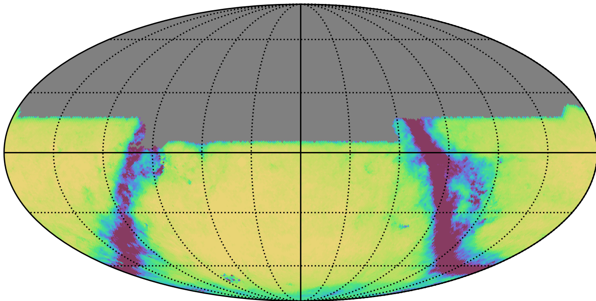
ddf_loaded_fl8_v3.4_10yrs All sky u band: Exgal_CoaddM5
