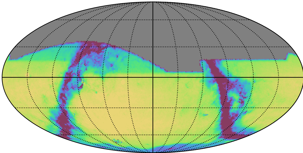
ddf_loaded_fl8_v3.4_10yrs All sky r band: Exgal_CoaddM5
