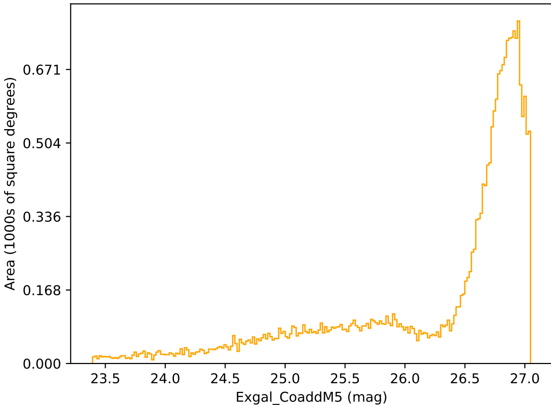
ddf_loaded_fl8_v3.4_10yrs All sky r band: Exgal_CoaddM5
