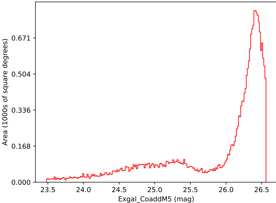
ddf_loaded_fl8_v3.4_10yrs All sky i band: Exgal_CoaddM5
