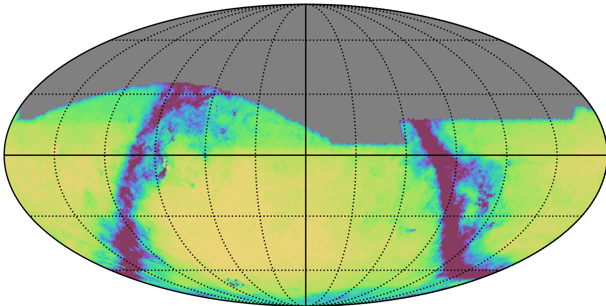
ddf_loaded_fl8_v3.4_10yrs All sky g band: Exgal_CoaddM5
