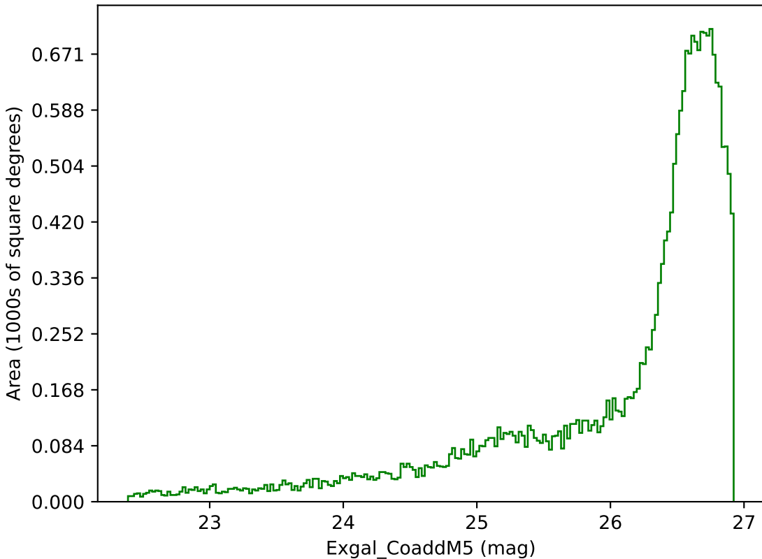
ddf_loaded_fl8_v3.4_10yrs All sky g band: Exgal_CoaddM5
