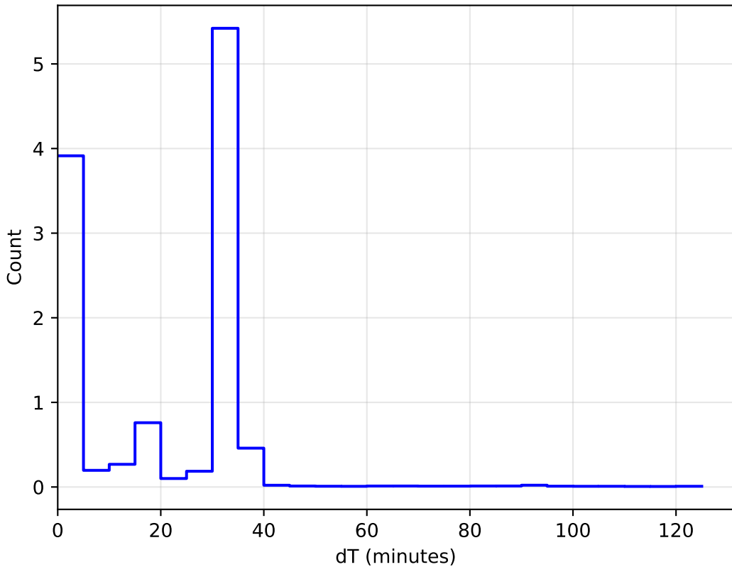
1e6 ddf_loaded_fl8_v3.4_10yrs WFD: DeltaT Histogram
