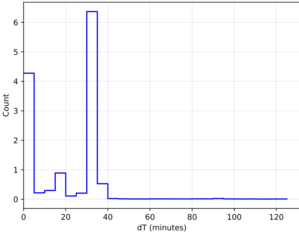
1e6 ddf_loaded_fl8_v3.4_10yrs All sky: DeltaT Histogram
