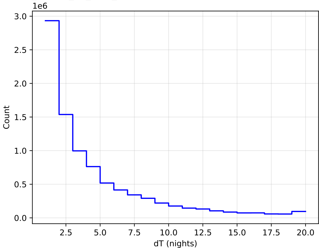
ddf_loaded_fl8_v3.4_10yrs All sky all bands: DeltaNight Histogram
