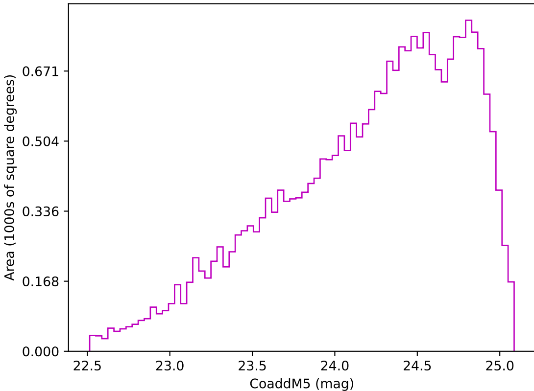
ddf_loaded_fl8_v3.4_10yrs Yr 3-4 z band: CoaddM5
