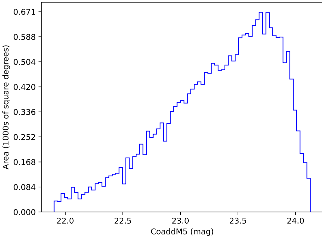
ddf_loaded_fl8_v3.4_10yrs Yr 3-4 y band: CoaddM5
