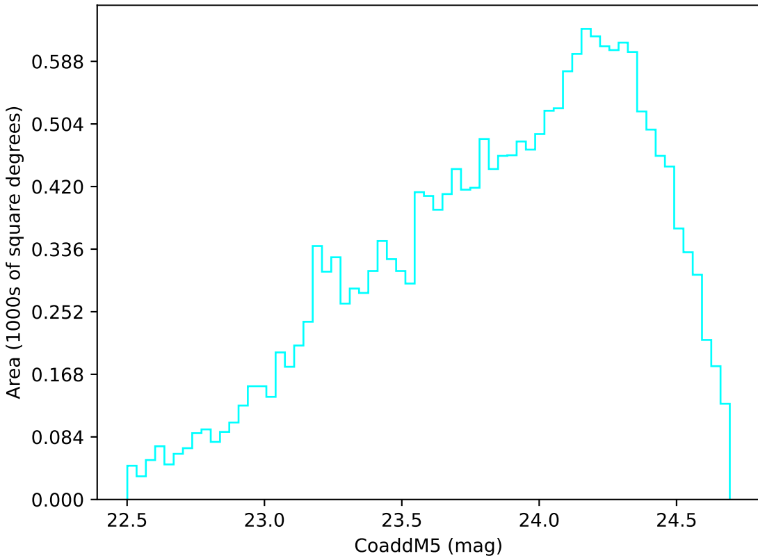
ddf_loaded_fl8_v3.4_10yrs Yr 3-4 u band: CoaddM5
