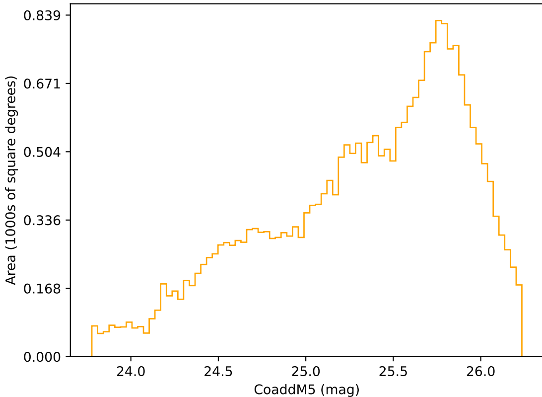
ddf_loaded_fl8_v3.4_10yrs Yr 3-4 r band: CoaddM5
